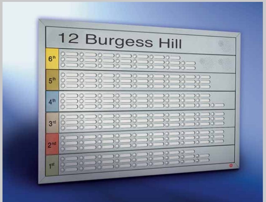
Fig. 32/2 Bespoke bell and intercom box with 40 mm aluminium plaster frame and RSA , with rear inspection panel.
