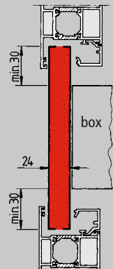
Front plate integrated in door profile
