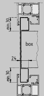
Front plate integrated in door profile
